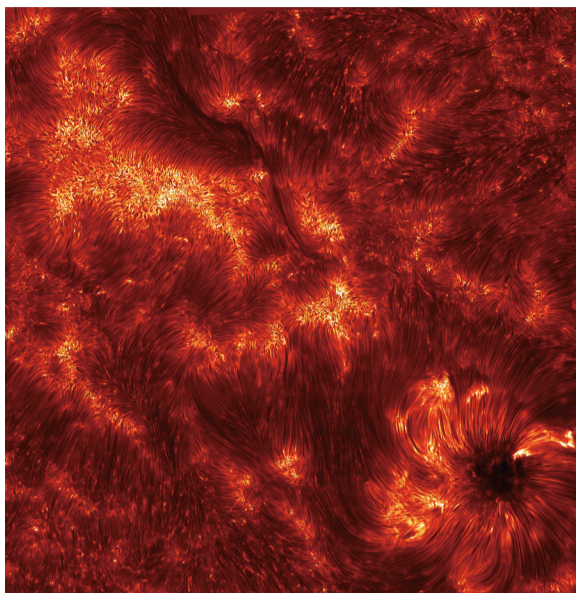
A solar active region observed in the core of the CaII line at 854.2nm with the IBIS imaging spectrometer.
